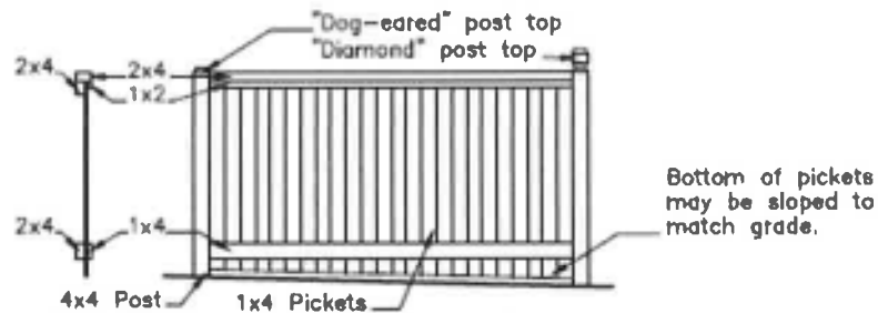
CROSS-SECTION OUTSIDE ELEVATION
